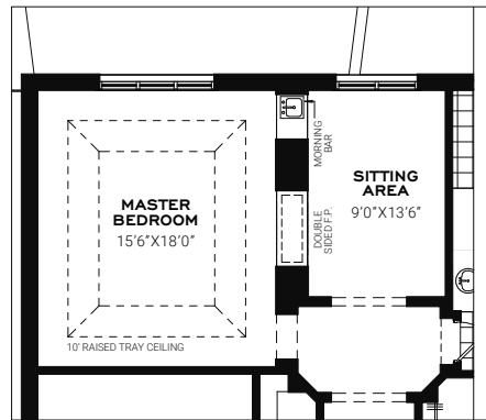
OPT. SECOND FLOOR DOUBLE-SIDED FIREPLACE
