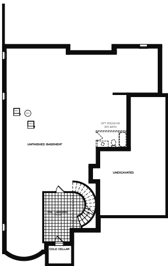
BASEMENT PLAN A
