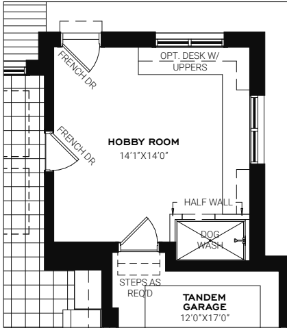
OPT. GROUND FLOOR DOG WASH
