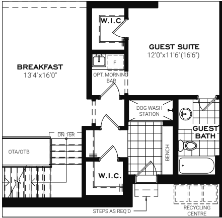
OPT. GROUND FLOOR DOG WASH
