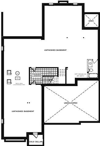
BASEMENT PLAN A
