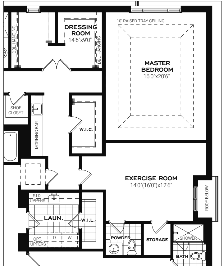
OPT. SECOND FLOOR EXERCISE ROOM
