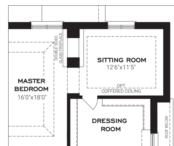
OPT. SECOND FLOOR WITH DOUBLE SIDED FIREPLACE (NOT AVAILABLE WITH 5 BEDROOM PLAN)
