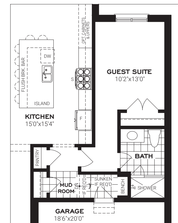
OPT. GROUND FLOOR WITH GUEST SUITE ADDITIONAL 197 SQ. FT.
