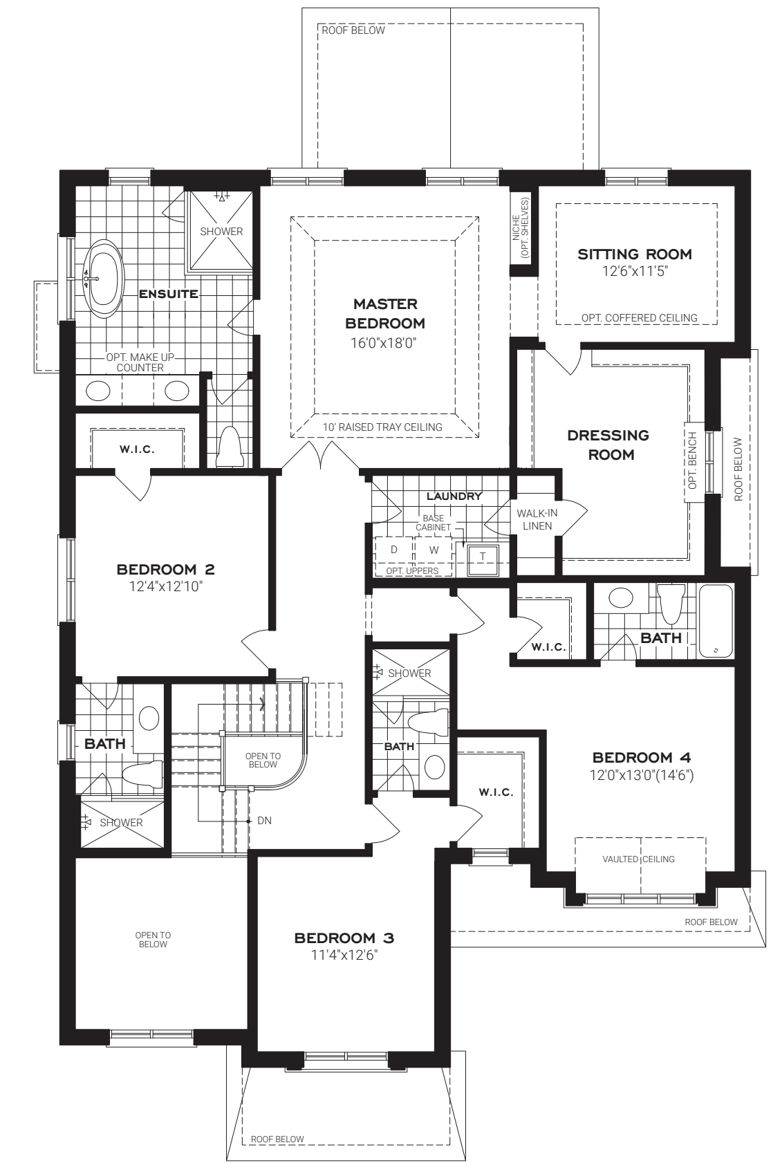
SECOND FLOOR PLAN A
