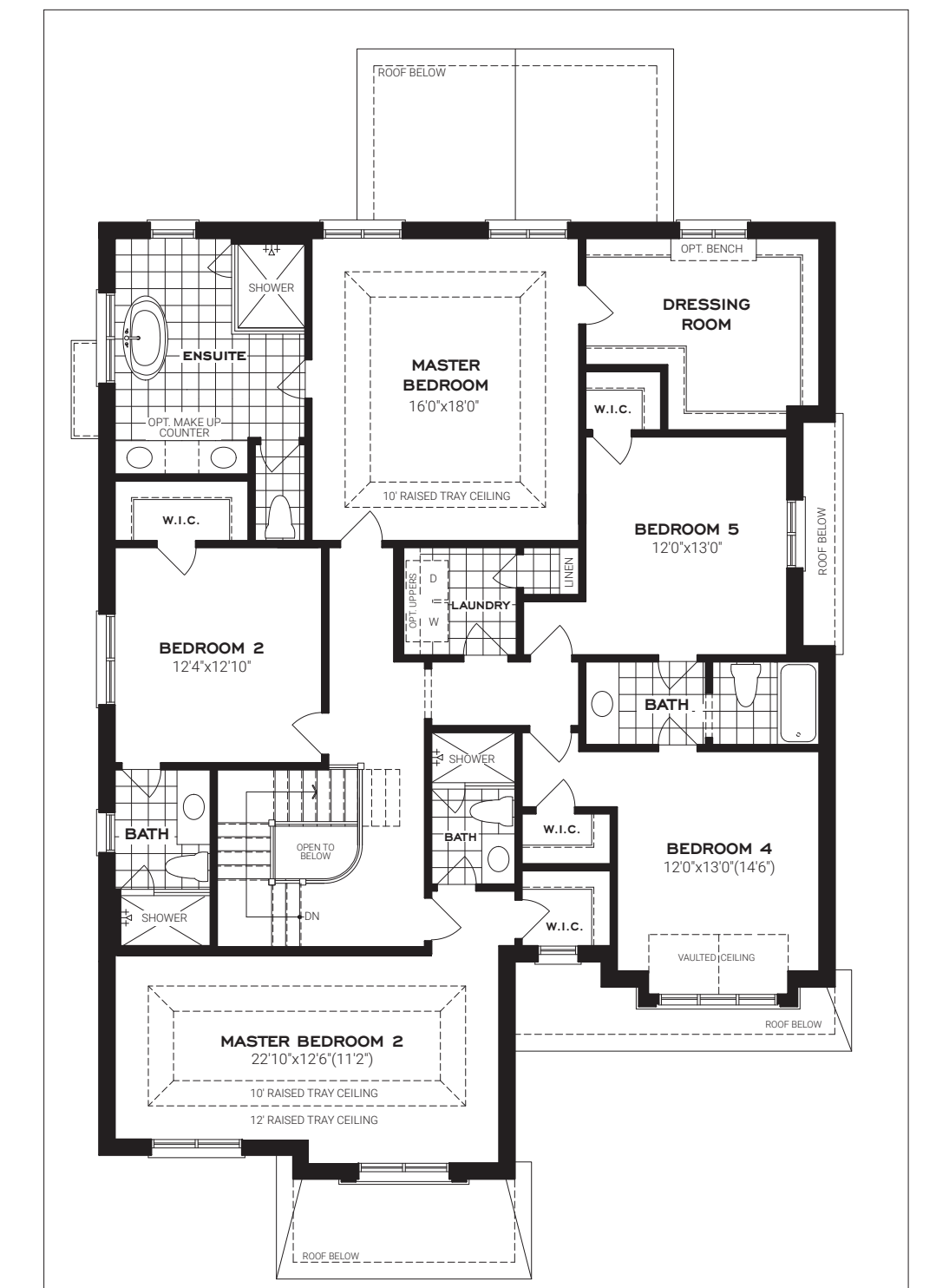
OPT. SECOND FLOOR ELEVATION A 5 BEDROOM PLAN WITH DUAL MASTER INCLUDES ADDITIONAL 121 SQ. FT.
