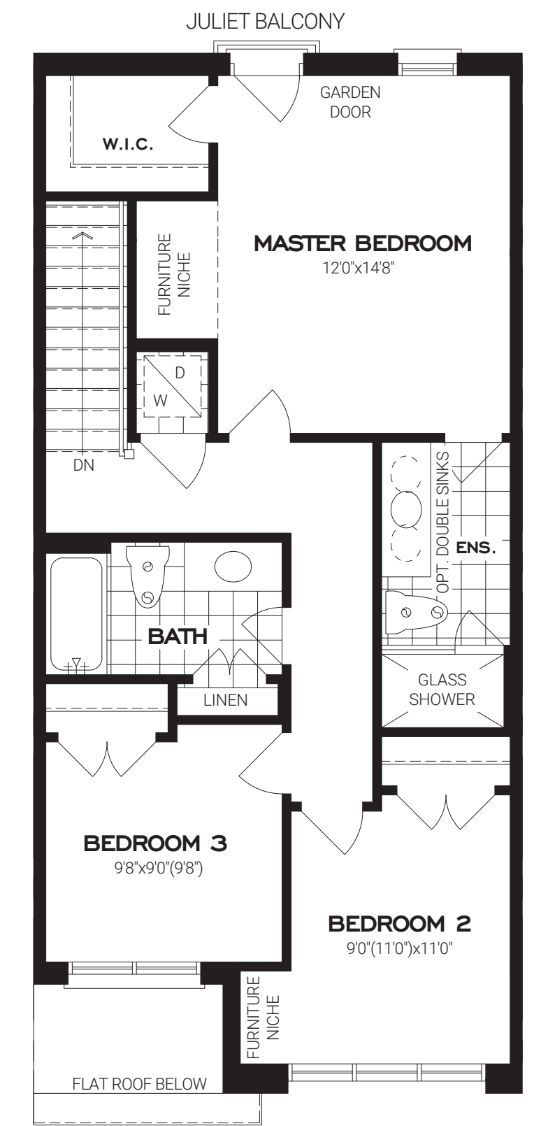
ALTERNATE THIRD FLOOR PLAN WITH 4 PC. MASTER ENSUITE
