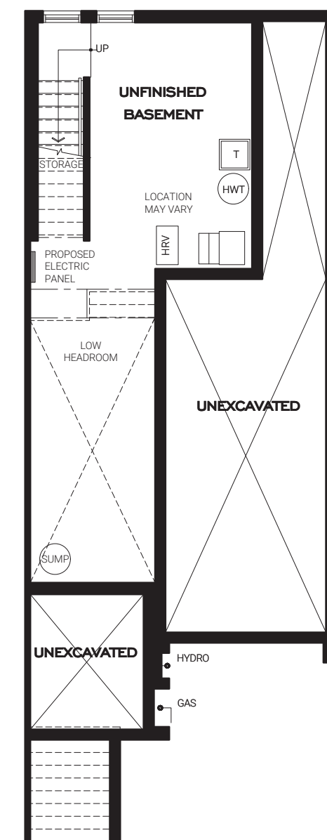
BASEMENT FLOOR PLAN A
