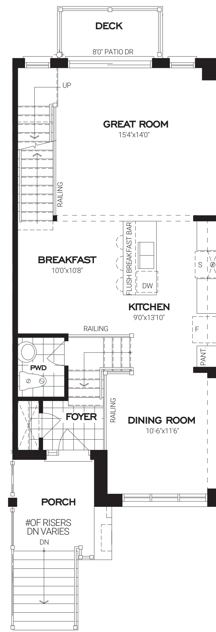
SECOND FLOOR PLAN A
