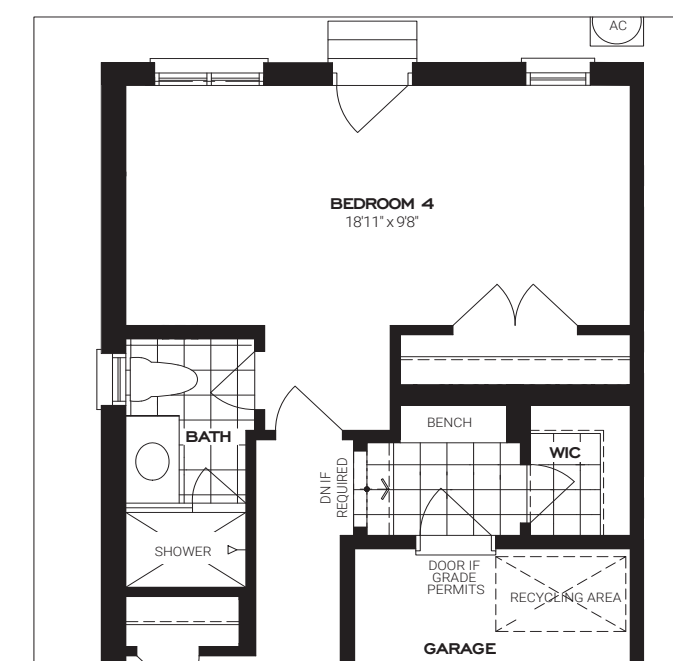
OPT. GROUND FLOOR
