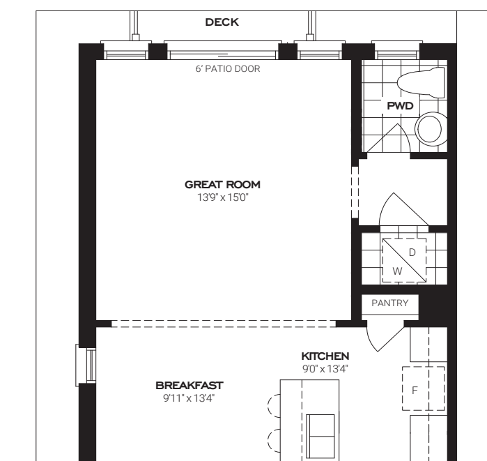
OPT. SECOND FLOOR
