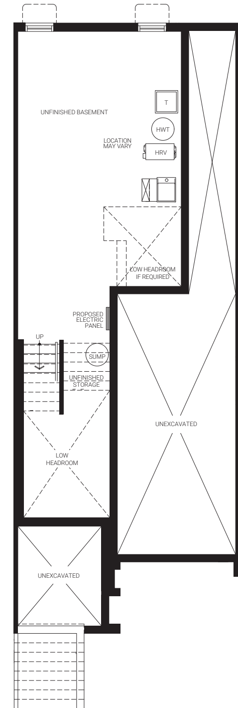
BASEMENT FLOOR PLAN A
