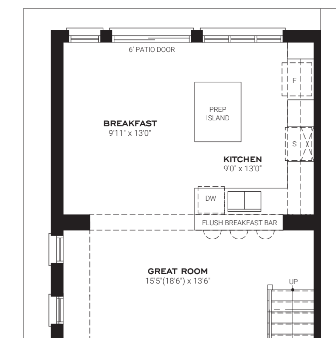
OPT. SECOND FLOOR
