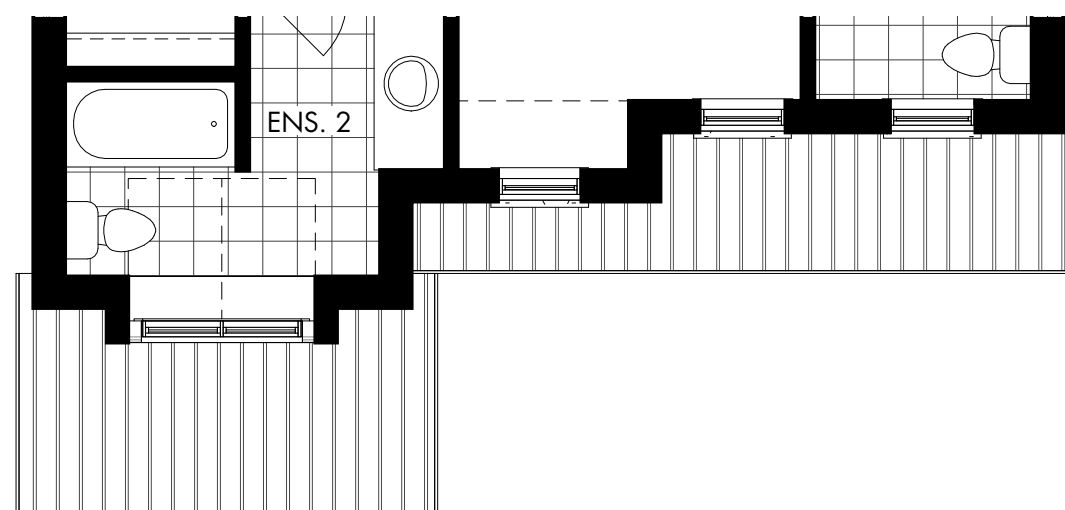
PARTIAL SECOND FLOOR ELEV. C
