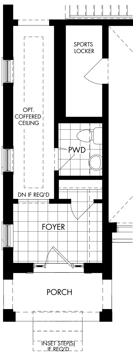
OPT. SPORTS LOCKER
