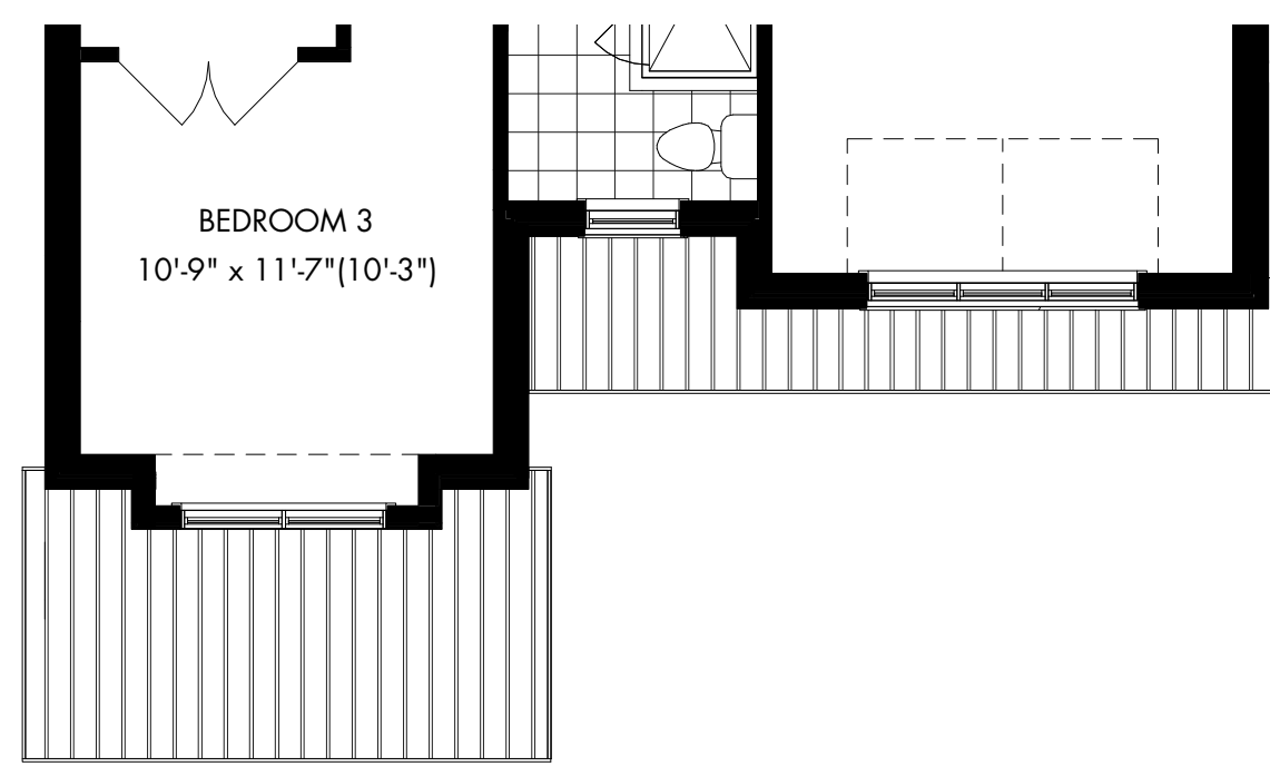
PARTIAL SECOND FLOOR ELEV. C
