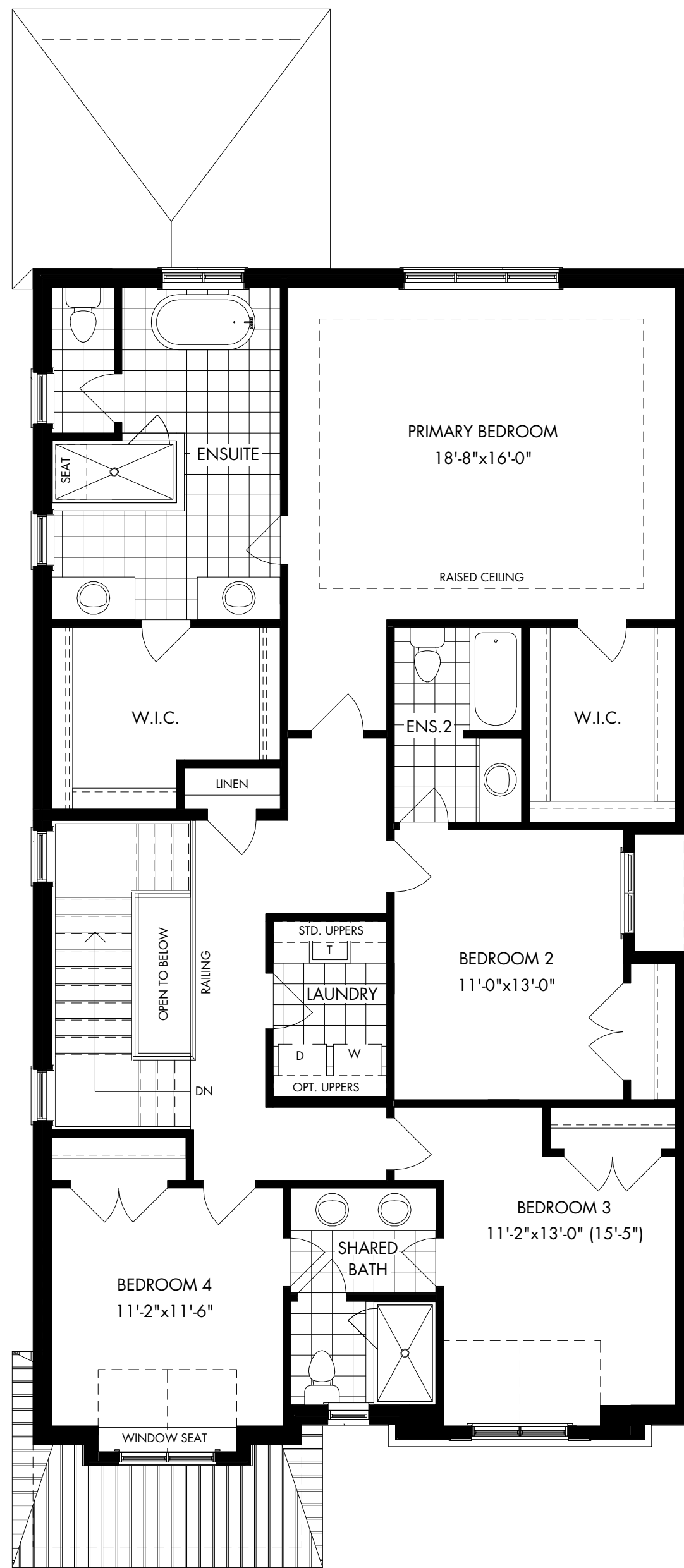
SECOND FLOOR ELEV. A
