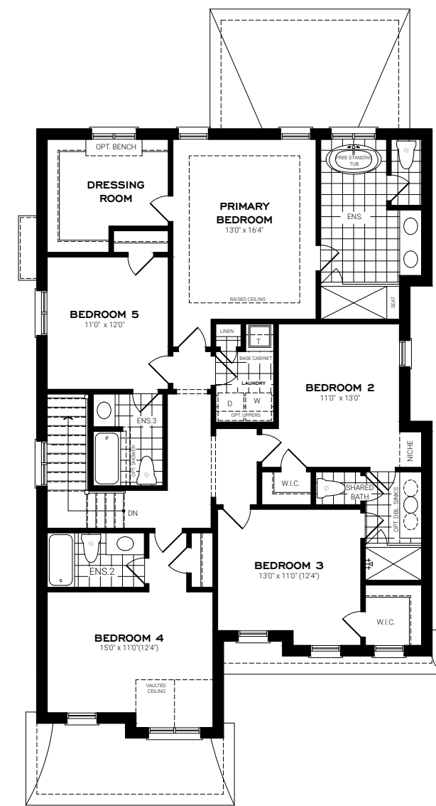
OPT. SECOND FLOOR A 5 BEDROOM
