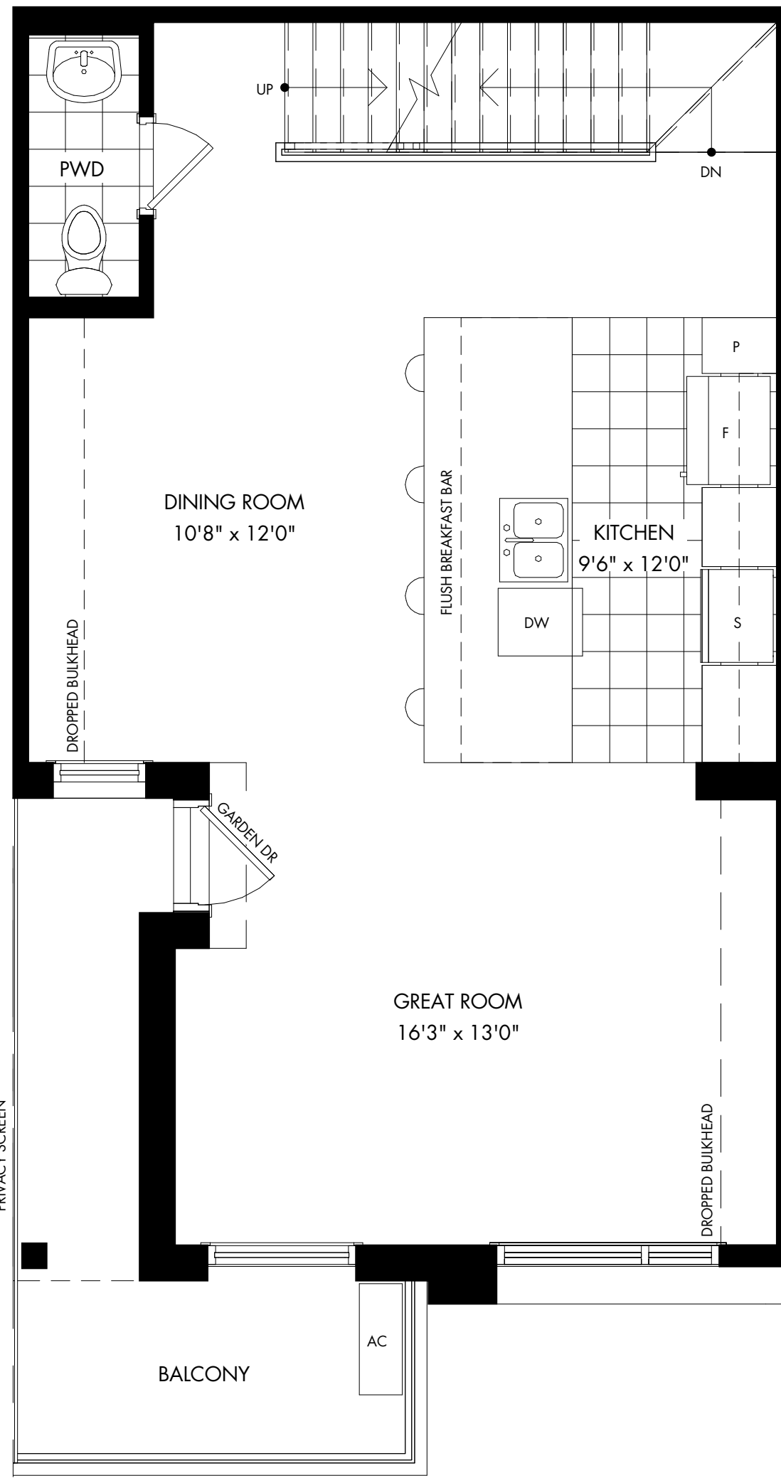
ALTERNATE FLOOR PLAN WITH LAUNDRY RELOCATED TO THIRD FLOOR
