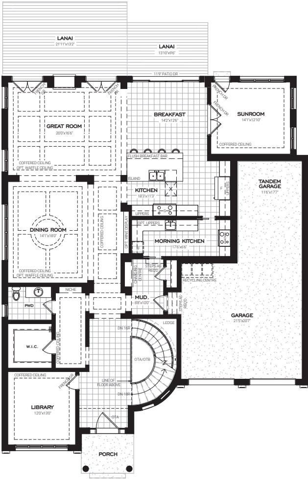
GROUND FLOOR PLAN B
