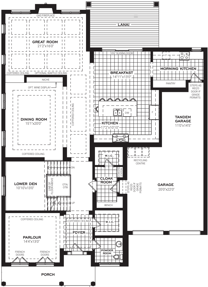
GROUND FLOOR PLAN A
