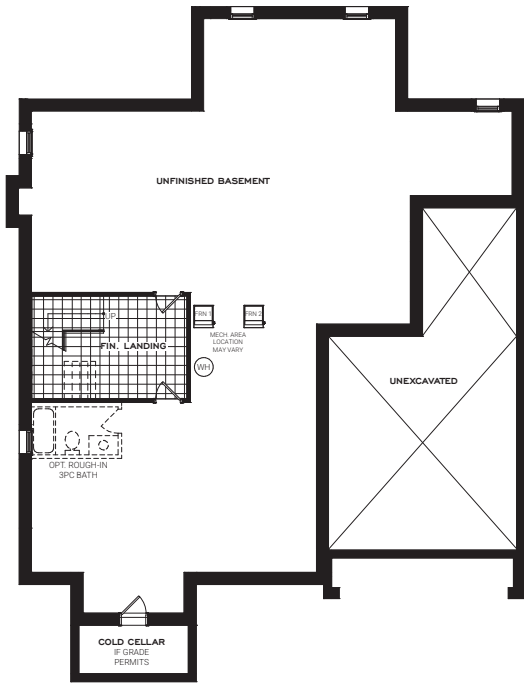
BASEMENT PLAN B
