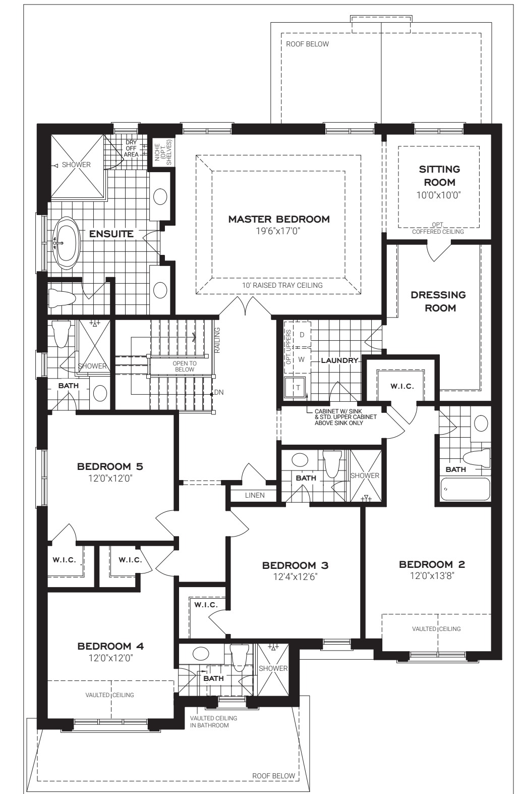
OPT. SECOND FLOOR ELEVATION A 5 BEDROOM PLAN
